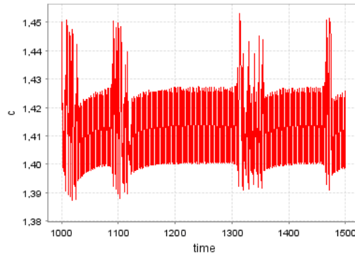
FIG. 14. model 1; trajectory of c_t [ k_0 = 8; d_0 = 0.25; \phi_0 = 0.3; \phi_1 = 2.5 ; transients=1000; iterations=500]
