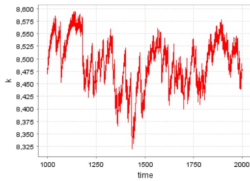
FIG. 10. model 1; trajectory of k_t [ k_0 = 8; d_0 = 0.25; \phi_0 = 0.3; \phi_1 = 0 ; transients=1000; iterations=1000]
