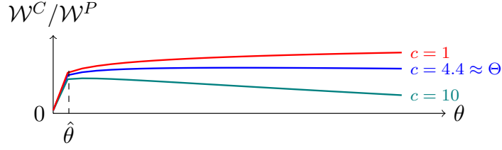
FIG. 1. Result (i) of Lemma 7: \alpha = 0.24 , \eta = 0.58 , r = 0.004 , \delta = 0.036 , p = 1 and \hat{\theta} \approx 0.44 .
