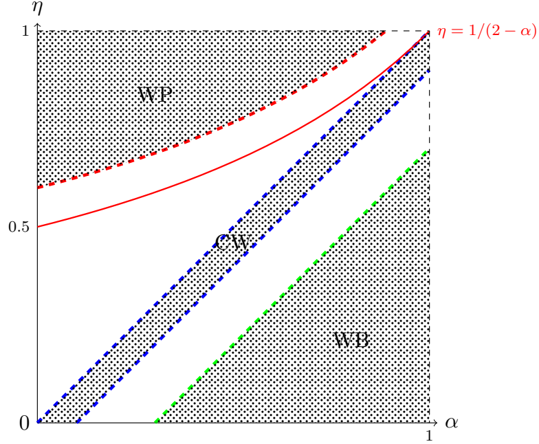
FIG. 2. Relative efficiency: \eta = \beta , r + \delta = 1 , p = 1 (normalization) and c > 1 .
