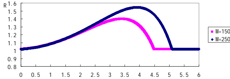
FIG. 1. Characteristics of bank lending ( M = 250, 150 )
